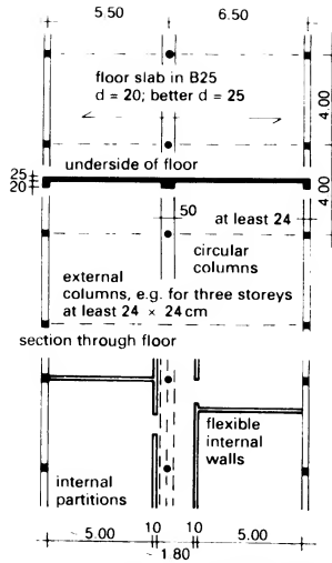
1 Structural system: asymmetrical double-span beams
